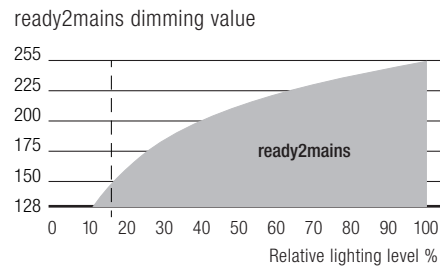
Dimming characteristics as seen by the human eye
